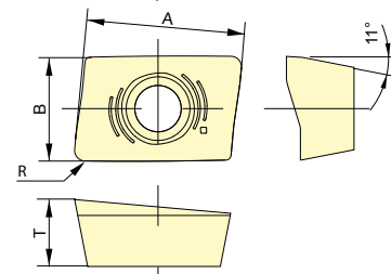
Fig.4 Sharp-edged insert
