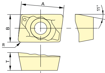
Fig.1 Wave-edged insert
